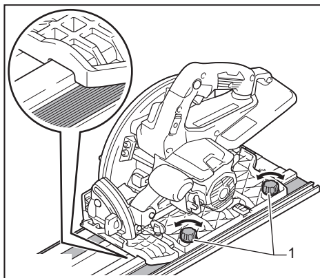
► 1. Adjusting screws
